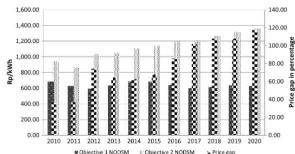
Fig. 7. Generating costs and percentage of price gap
