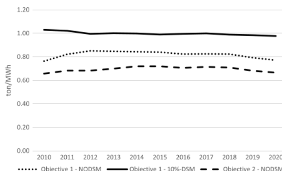
Fig. 6. Emissions intensity (t/MWh) subcritical scenario, minimizing generating costs
