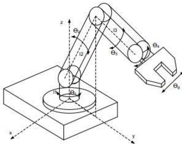
Gambar 3.4 menunjukkan model robot Manipulator Sendi Lengan ( Joint - Arm )
