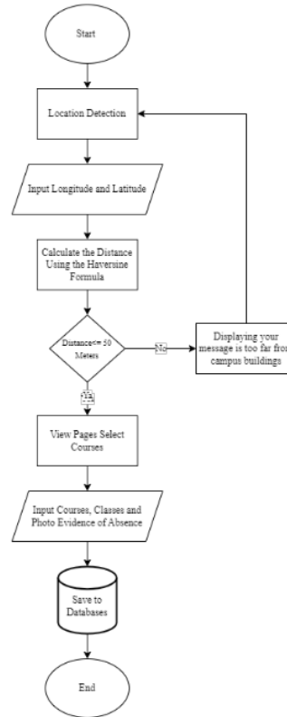
Fig. 2. Haversine Formula Algorithm Flowchart
