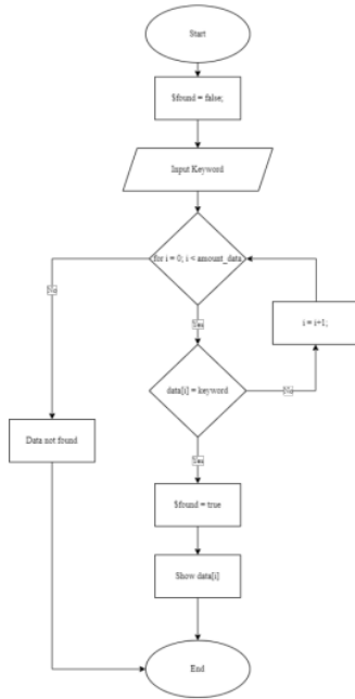
Fig. 3. Sequential Search Algorithm Flowchart
