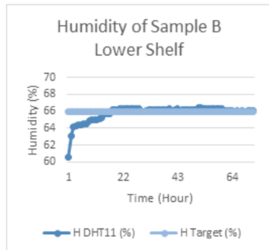
1 Fig 15. The Humidity of storage box with sample bags B inside
