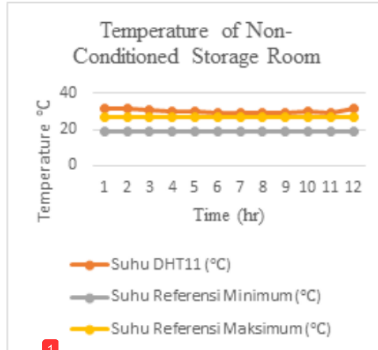
Fig 10. Temperature in storage box to outside box
