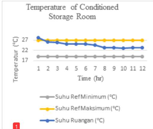
Fig 8. Temperature in conditioned storage box
