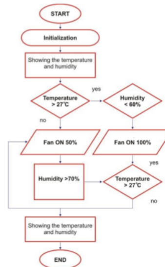
Fig 2. Flow chart System
