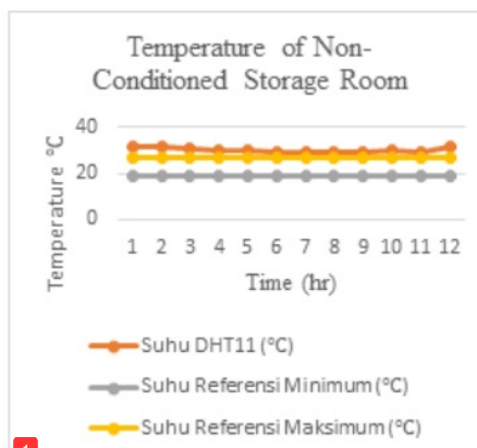
Fig 6. Temperature In Non-Conditioned Storage Box
