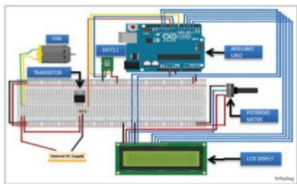
Fig 3. Wiring diagram of circuit used for controller
