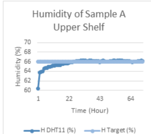
1 Fig 14. The Humidity of storage box with sample bags A inside
