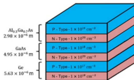
Figure 3: The simulation of triple-junction solar cell modelling
