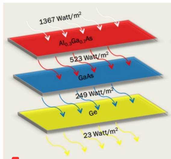
Figure 2: The simulation result of triple-junction solar cell transmission intensity
