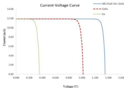
1 Figure 6: Current-Voltage Curve of Solar Cell
