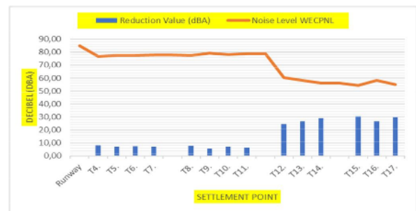
Figure 9: Noise level and zone coverage reduction value
