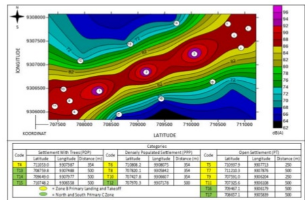
Figure 6: Noise Distribution (LDN)
