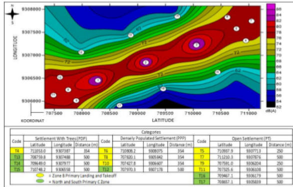
Figure 7: Noise Distribution (WECPNL)
