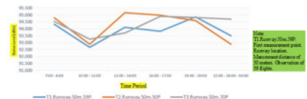
Figure 3: The noise level on the runway
