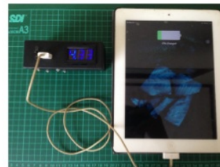
Fig. 20. Charging test of Ipad Gen 2.
