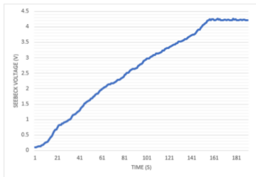
Fig. 15. Seebeck voltage on time.
