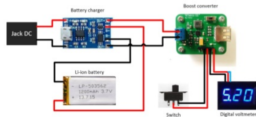
Fig. 11. Electronic unit wiring diagram.
