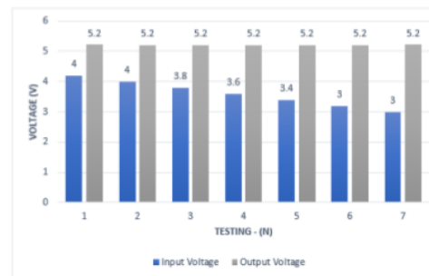
Fig. 16. Graph of boost converter testing.
