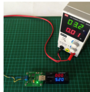
Fig. 17. Boost converter testing.
