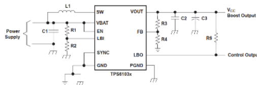
Fig. 4. Boost converter circuit of IC TPS61030 [16].
