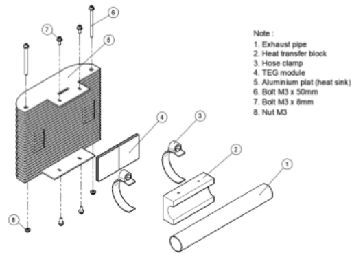
Fig. 6. Construction of harvester unit.
