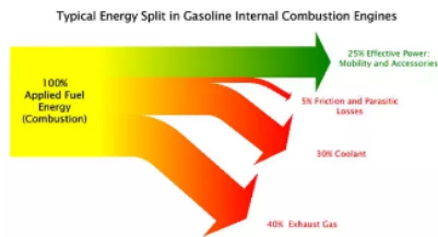
Fig. 2. Diagram Sankey of ICE [14].
