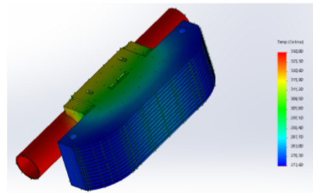
Fig. 7. Temperature distribution simulation of a harvester.
